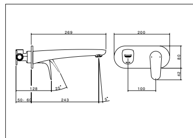
flickmixer plus wall bath mixer 240mm 4552.04
