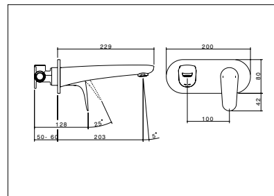
flickmixer plus wall basin mixer 200mm 4551.045A
