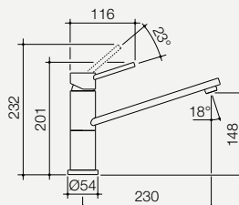
Villa Sink Mixer 6905.914A Available in chrome 6905.044A WELS 4 Stars Rated, 7.5L/min
