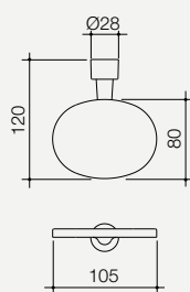
Villa Soap Dish 6915.04 Chrome Only
