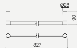
Villa Single Towel Rail 6911.91 Available in chrome 6911.04
