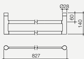
Villa Double Towel Rail 6912.91 Available in chrome 6912.04
