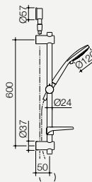
Villa 2.0 Multifunction Rail Shower 6923.913A Available in chrome 6923.043A WELS 3 Stars Rated, 9L/min
