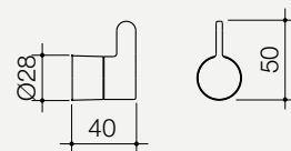
Villa Robe Hook 6910.91 Available in chrome 6910.04
