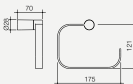
Villa Toilet Ring 6913.91 Available in chrome 6913.04
