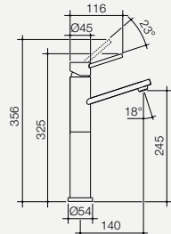
Villa Tower Basin Mixer 6902.915A Available in chrome 6902.045A WELS 5 Stars Rated, 6L/min
