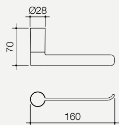
Villa Toilet Roll Holder 6909.91 Available in chrome 6909.04
