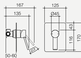
Villa Bath/ Shower Mixer 6903.91 Available in chrome 6903.04
