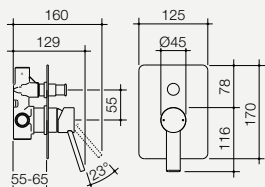
Villa Bath/ Shower Mixer with Diverter 6904.91 Available in chrome 6904.04
