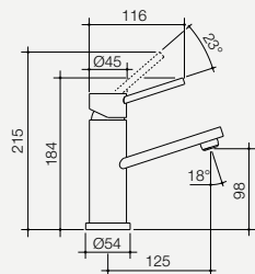
Villa Basin Mixer 6901.915A Available in chrome 6901.045A WELS 5 Stars Rated, 6L/min
