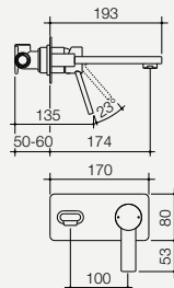
Villa Wall Basin/ Bath Mixer 6906.915A Available in chrome 6906.045A WELS 5 Stars Rated, 6L/min
